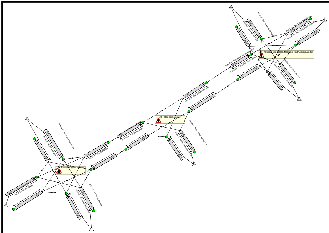
Figure 3.2: Modelled LinSig network
